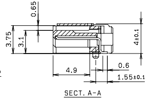
SECT. A-A
